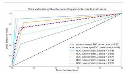
(b) Three layer BPNNet-ROC
