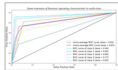
(a) Two layer BPNNet-ROC
