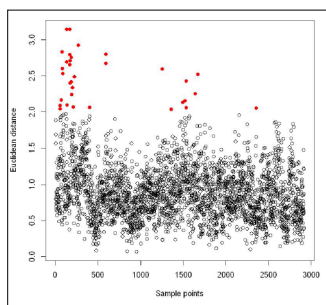
Figure 5: Diagram of outliers.
