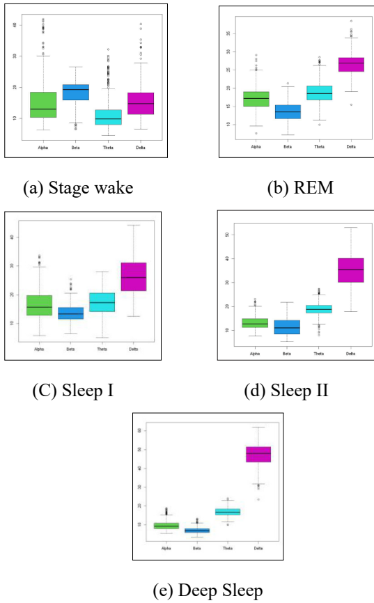
Figure 4: Boxplot of each sleeping period.
