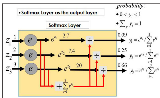
Figure 3: Principle of Softmax function
