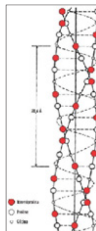
COLLAGEN STRUCTURE
